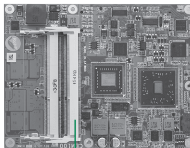
Double deck DDR3 SO-DIMM
