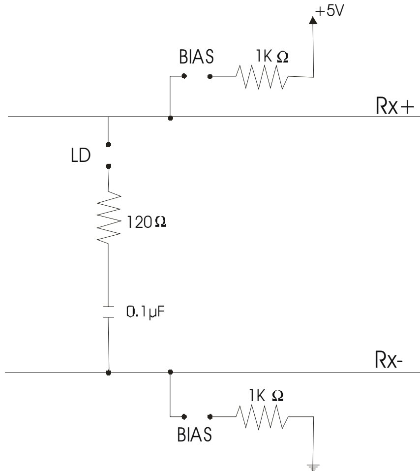
Figure 3-1: Simplified Termination Schematic
