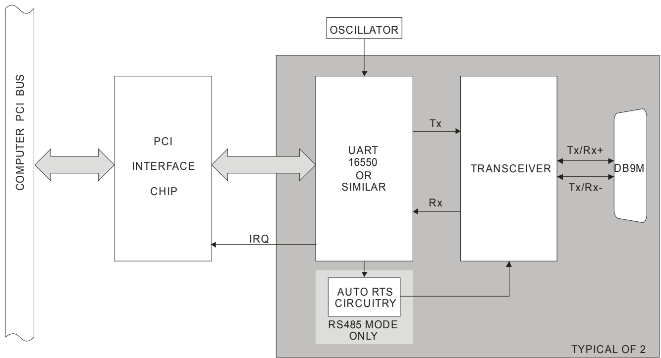
Figure 1-1: Block Diagram
