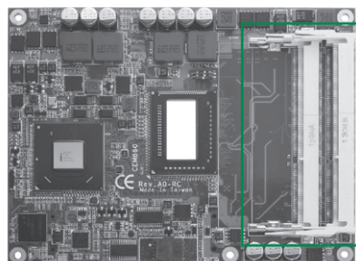
Double deck DDR3 SO-DIMM
